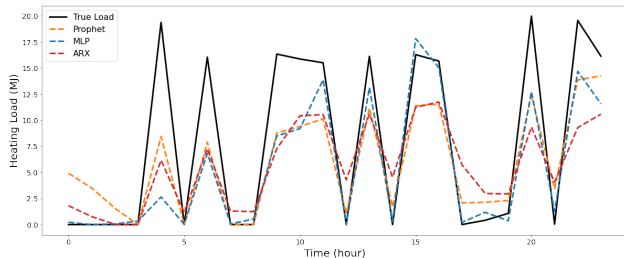
Figure 2. Model performance comparison on a 24-hour forecasting horizon from the test set. Black solid line represents true load, and the dashed orange, red and blue lines are from Prophet, ARX, and MLP models respectively. Compared to Prophet and ARX, MLP can better capture extreme load conditions such as peaks. Nonetheless, Prophet and ARX correctly forecast general load trend.
