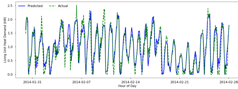
(a) 1 Hour Ahead Heat Load Predictions
