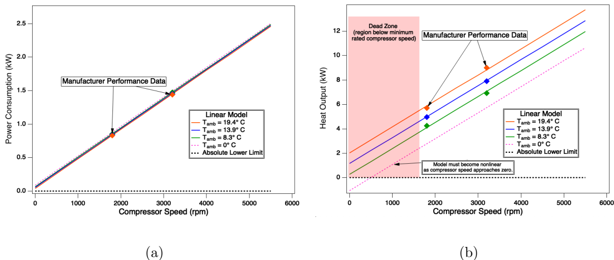
Figure 1: VSHP performance curves at T_{indoor} = 21.1^{\circ}C for (a) power consumption and (b) heat output. The shaded dead zone in (b) shows where the model breaks down and gives unrealistic heat output at zero compressor speed. (Print in color)
