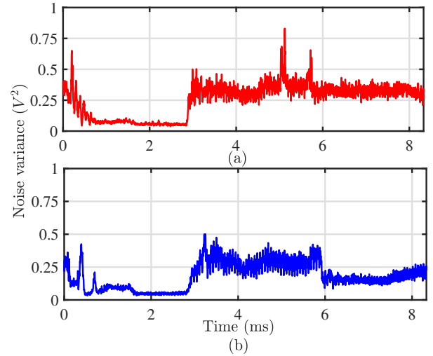
Fig. 11. Neutral-earth power-line noise variance measured at an electrical outlet in the FCIL microgrid. (a) FCIL microgrid operating in grid-connected mode. (b) FCIL microgrid operating in islanded mode.
