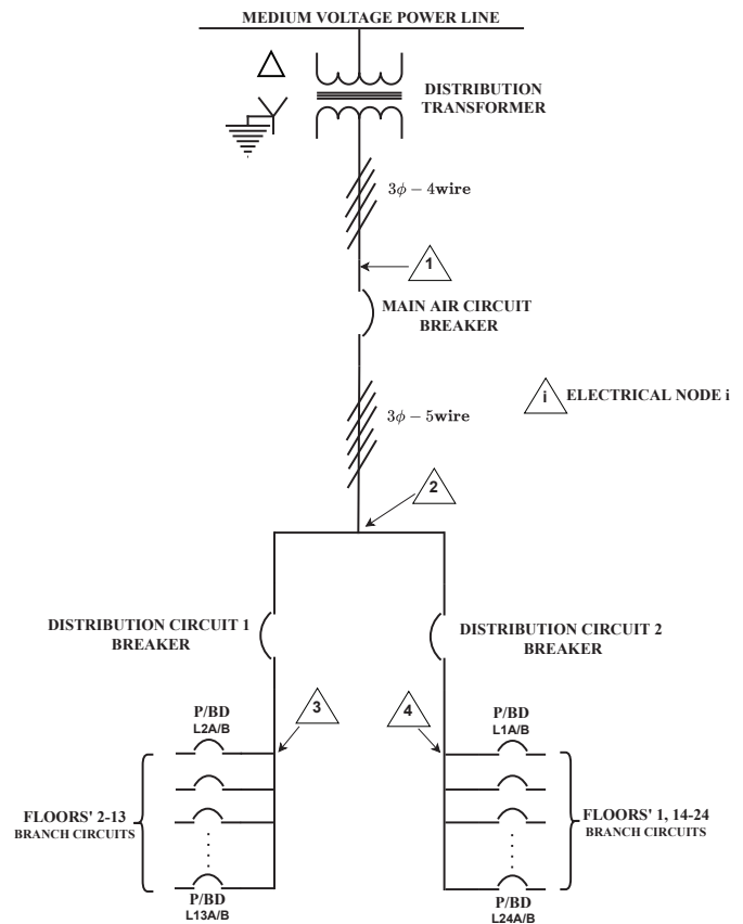
Fig. 9. Electrical circuit diagram of a 24-floor apartment building on the MIT campus.
