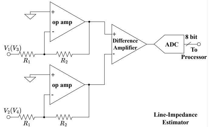
Fig. 6. Line-impedance estimator.
