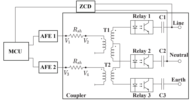
Fig. 2. Simplified circuit diagram of developed PLC modem.
