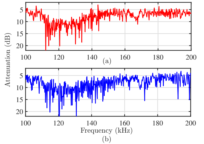
Fig. 13. Observed attenuation in FCIL microgrid. (a) FCIL microgrid operating in grid-connected mode. (b) FCIL microgrid operating in islanded mode.
