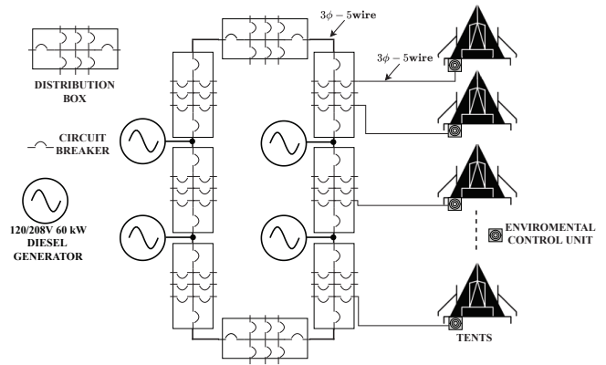
Fig. 8. Electrical circuit diagram of a military forward operating base operating as an islanded microgrid.
