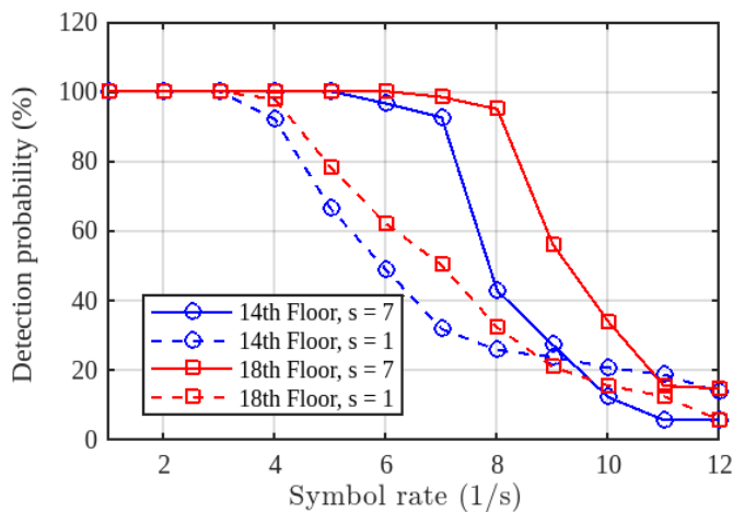
Fig. 19. Reliability of different time slots with different noise power. The PLC transmitter is located on the 14th and 18th floor, while the receiver is located on the 24th floor.
