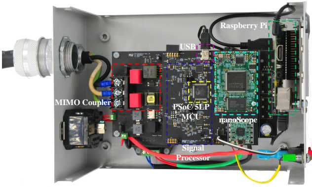
Fig. 1. Top view of the hardware including PLC modem and Raspberry Pi.
