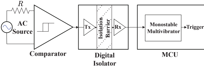
Fig. 3. AC mains voltage zero-crossing detection circuit.
