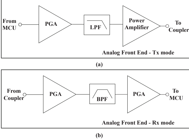
Fig. 4. AFE032 analog front-end circuit in (a) transmitter mode and (b) receiver mode.
